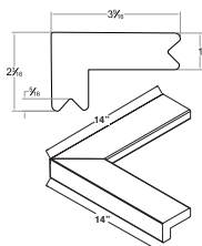
9979 Pre-fab Corner
